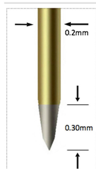
Needle Insulation
